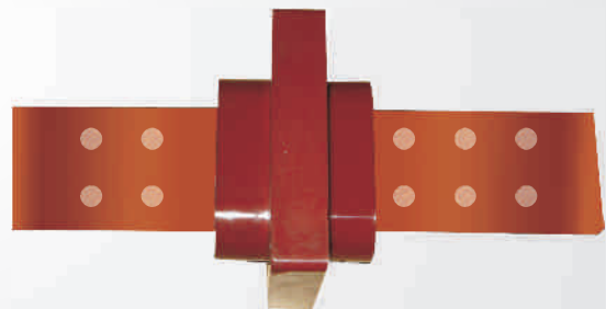
LV Bushing with Copper Flat moulded Options for flat sizes available for use upto 3150 Amps
